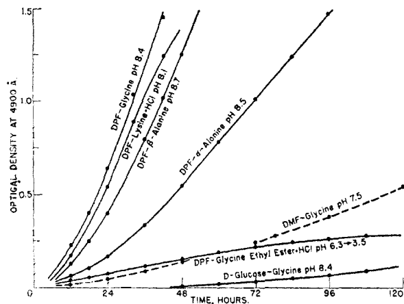
Fig. 1.—Rate of browning of 0.2 M aqueous solutions of 1-deoxy-1-piperidino-D-fructose (DPF), 1-deoxy-1-morpholino-D-fructose (DMF) and D-glucose with amino acids (2.0 M ) at 25°. The solution containing \alpha -alanine was saturated and a small amount remained undissolved.
