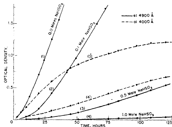
Fig. 2.—Effect of sodium bisulfite in delaying the browning reactions of 1-deoxy-1-piperidino-D-fructose (0.2 M ) with glycine (2.7 M ) at 25°. The molar concentrations of sodium bisulfite are given per mole of DPF.
